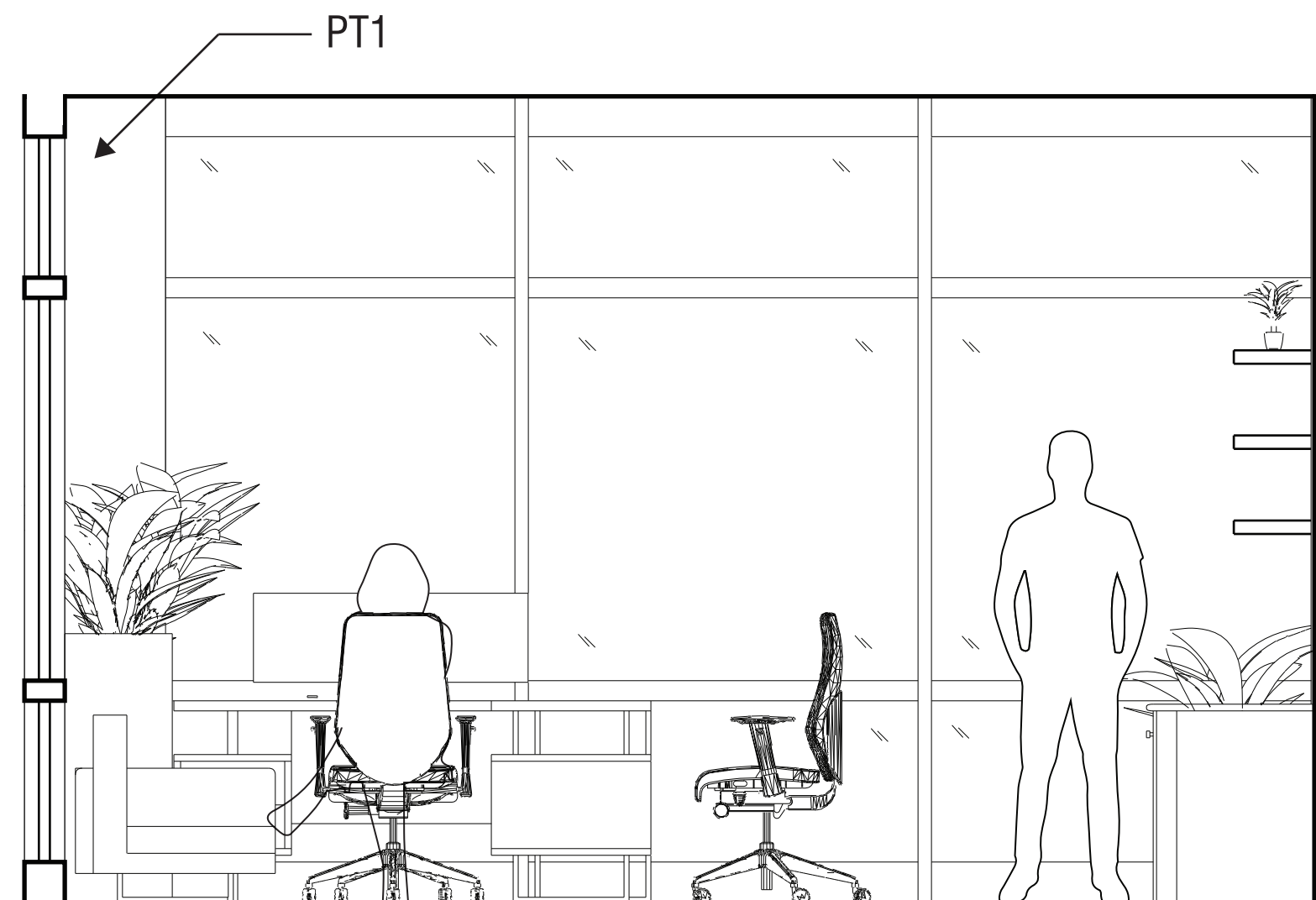
C ELEVATION C SCALE 1/2" - 1'-0"
