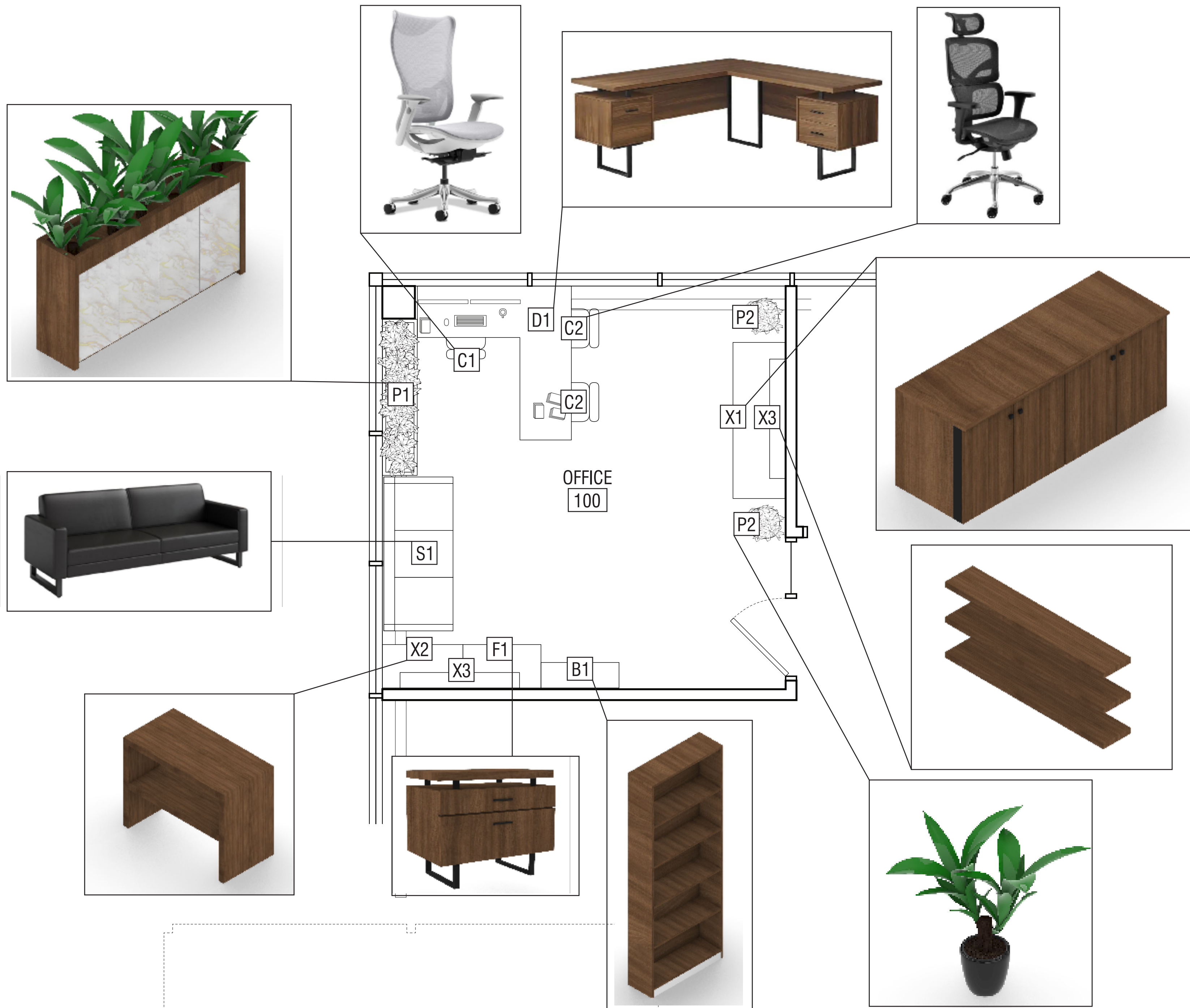
FURNITURE PLAN SCALE 3/8" - 1'-0"
