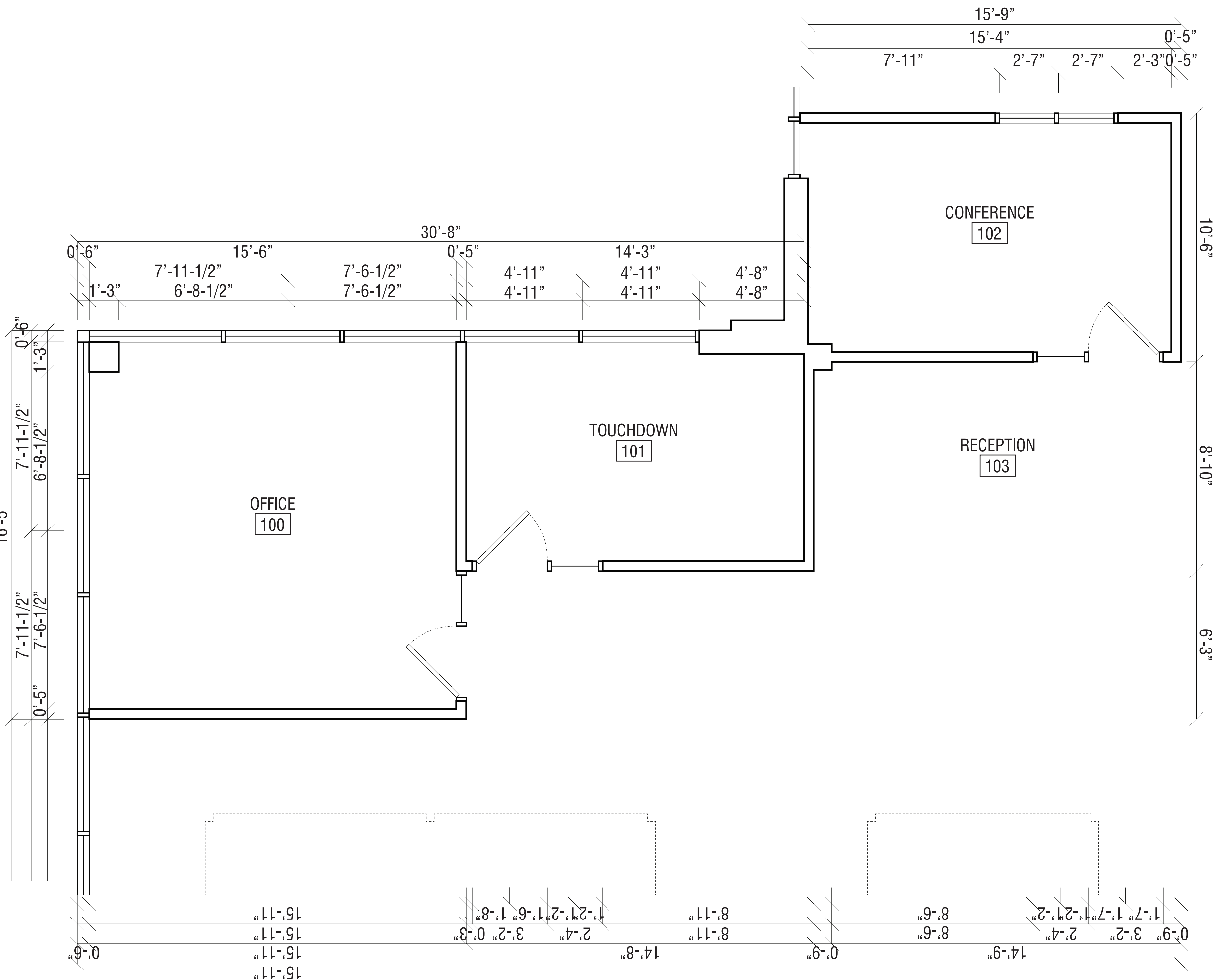
FLOOR PLAN SCALE 3/8" - 1'-0"
